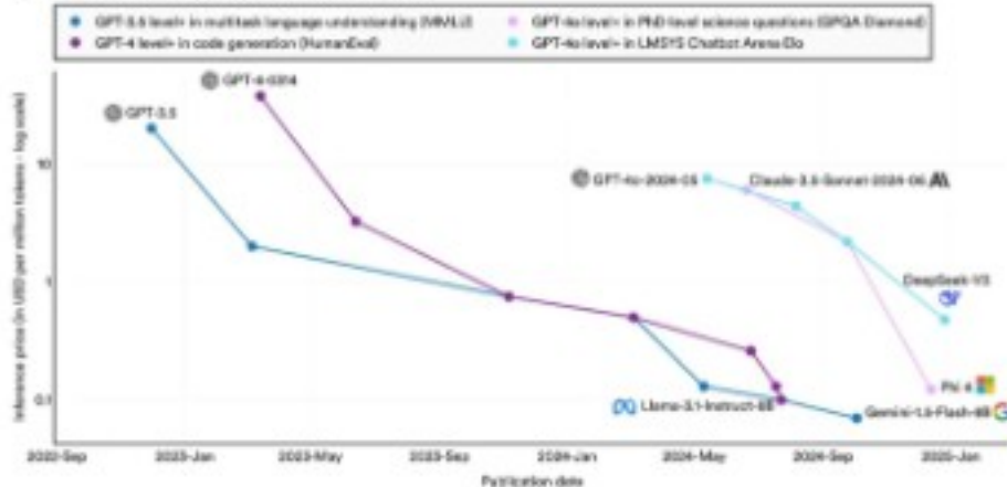
Inference price across select benchmarks, 2022-24
